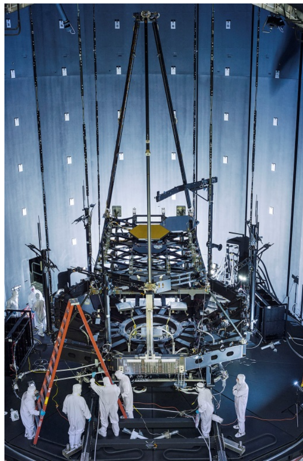
FIGURE 3.1.1 Major structural components of the James Webb Space Telescope being prepared for a cryogenic test. SOURCE: Courtesy of NASA/Chris Gunn.
