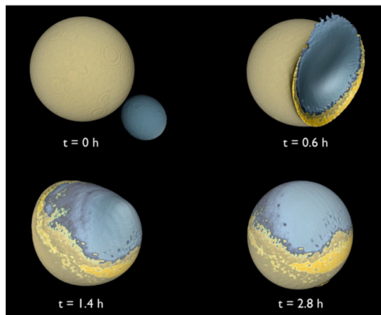
FIGURE 3.5.1 Theory and modeling are an important component of the scientific enterprise. Illustrated here are four time steps from a complex, three-dimensional computer simulation of an impact between the Moon and a hypothetical satellite, roughly 4-billion-years ago. SOURCE: Courtesy of Erik Asphaug (Arizona State University) and Martin Jutzi (University of Bern).
